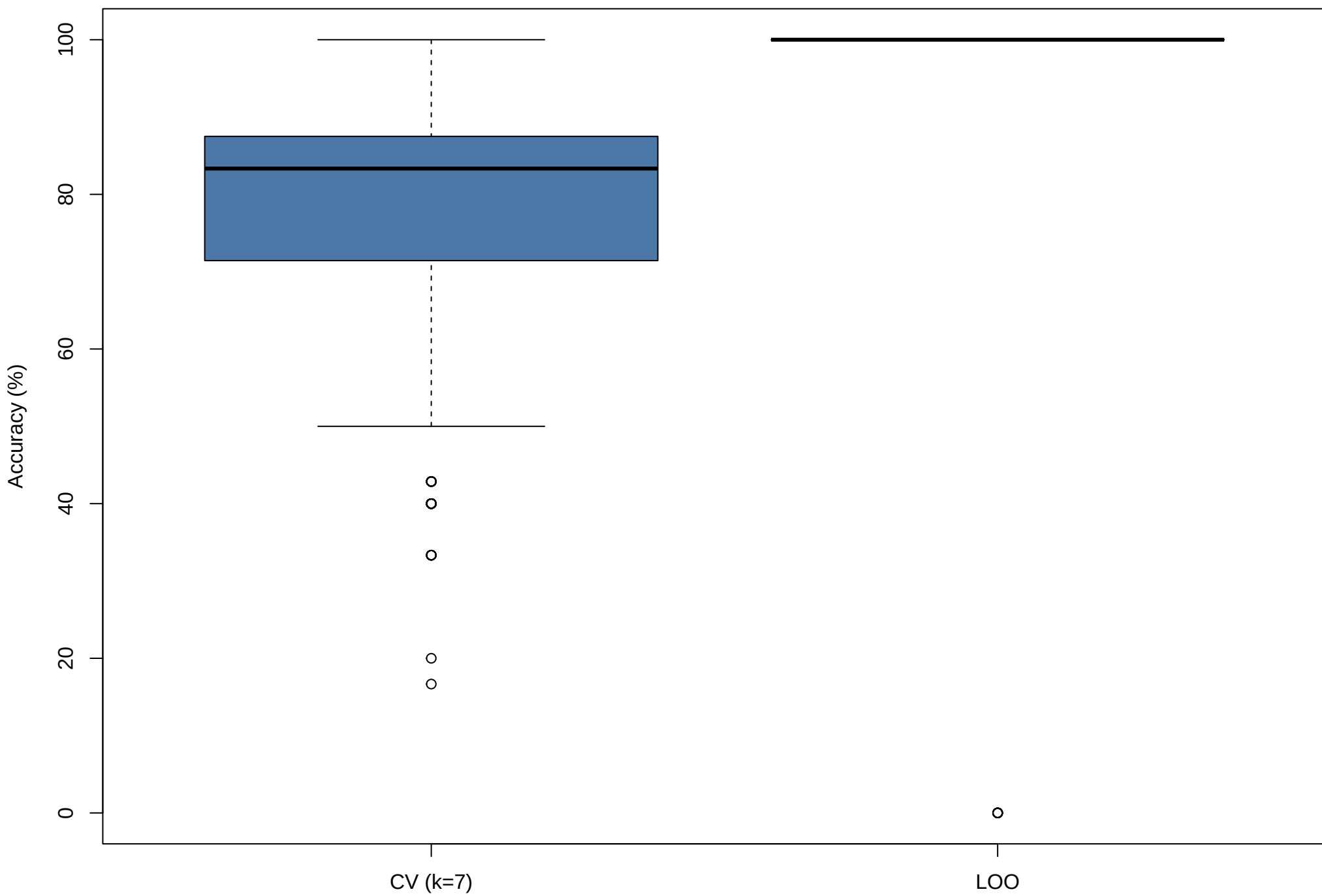
Cross-validation accuracy (class_weight)
